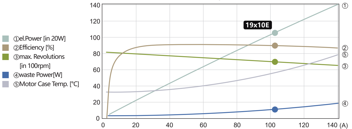
Motor Characteristics
